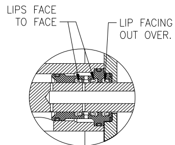
NOTE POSITION OF LIP SEALS
