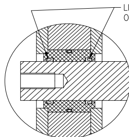
NOTE POSITION OF LIP SEALS
