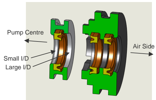
Lip Seal Positions
