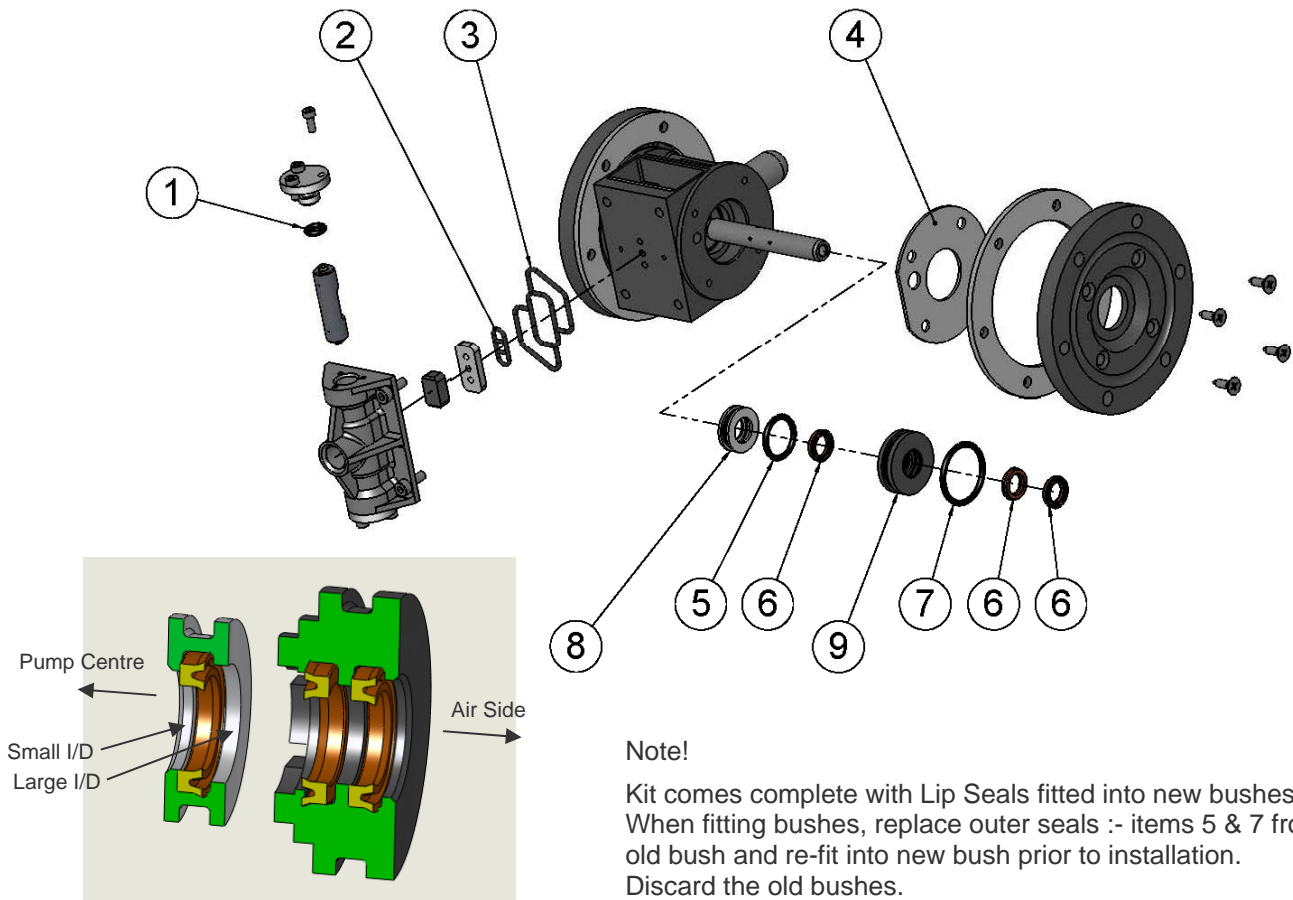
Lip Seal Positions
