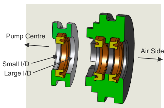
Lip Seal Positions
