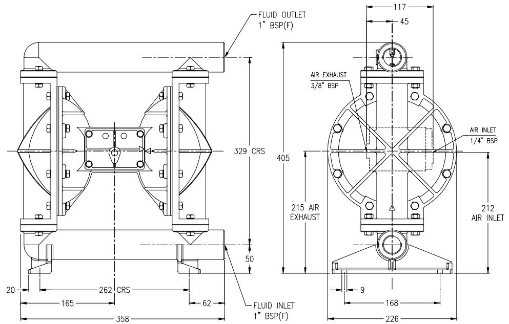
General Assembly :- B2502 Metallic pump All dimensions +/- 3mm
